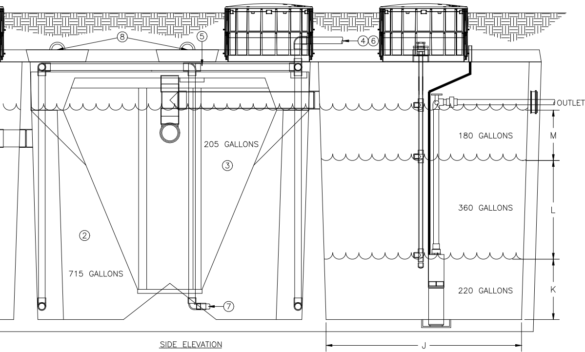
SIDE ELEVATION
