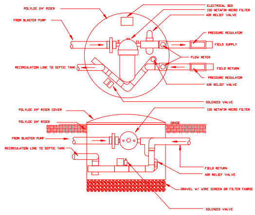
HOOT REMOTE HEADWORKS BOX DETAIL
